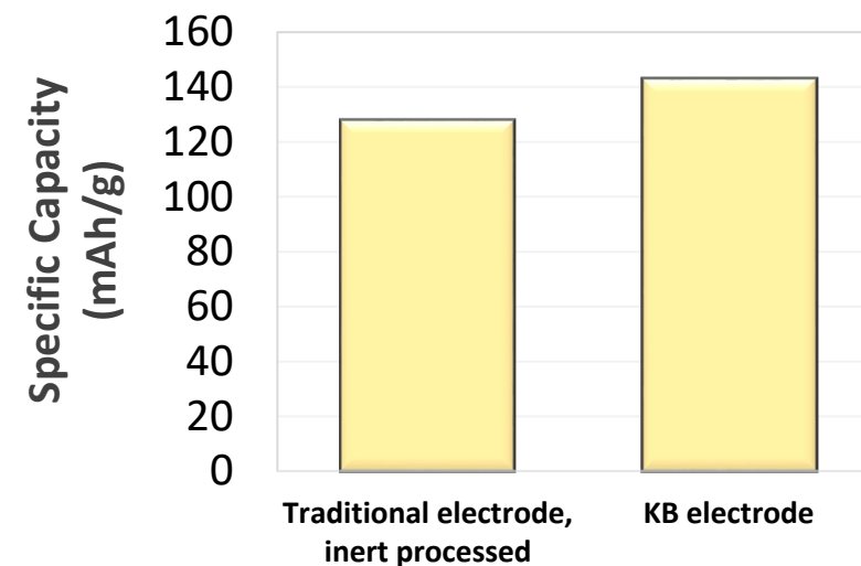
Half Cell Specific Capacity Comparison at \sim C/10
