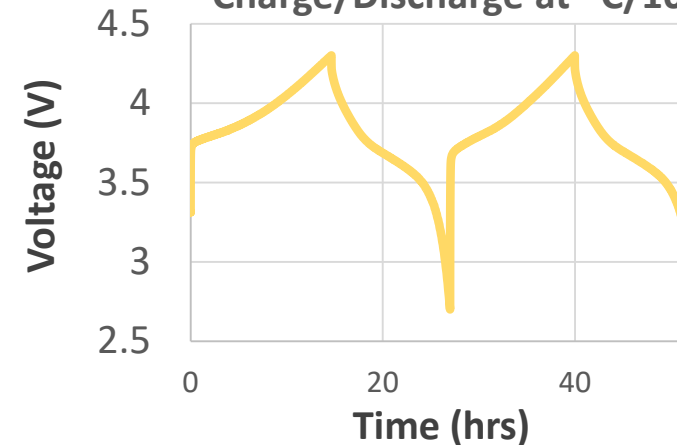
KB Cathode Half-Cell Charge/Discharge at \sim C/10
